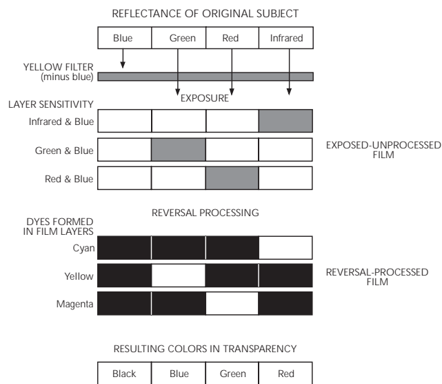
Figure 2: Color Reproduction of Typical Terrain with EKTACHROME Infrared Film
